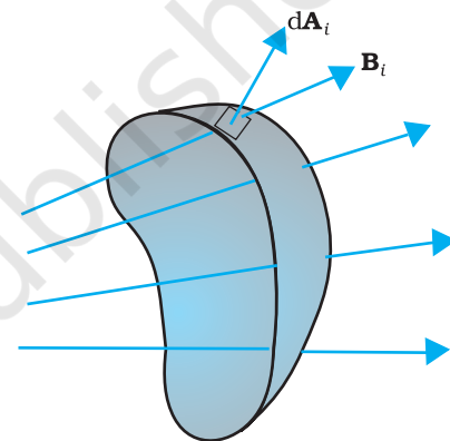
FIGURE 6.5 Magnetic field B_i at the i^{\text{th}} area element. d\mathbf{A}_i represents area vector of i^{\text{th}} area element.
