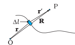
Line charge \Delta Q = \lambda \Delta l
